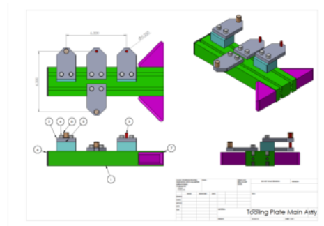
ASSEMBLY DRAWINGS
